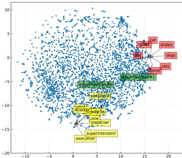
Figure 1: t-SNE projection of word/sense embeddings. Green labels show the two sense embeddings for dogy-chairman , whereas yellow and red labels show the nearest neighbours for the two senses. Best viewed in colour.
